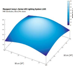
Maxspect Jump L-Series LED Lighting System L165 PAR Distributor, 90cm/24in above
