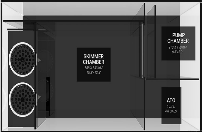
MARINE X 90.3 & 110.4 SUMP FILTRATION
